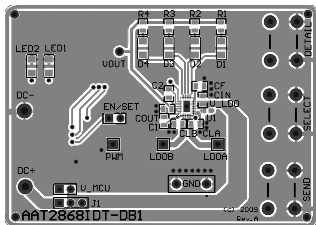
Figure 7: AAT2868 Evaluation Board Top Side Layout.
