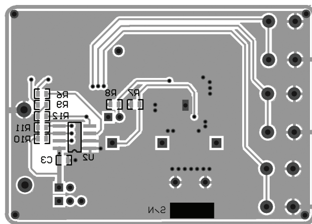
Figure 8: AAT2868 Evaluation Board Bottom Side Layout.
