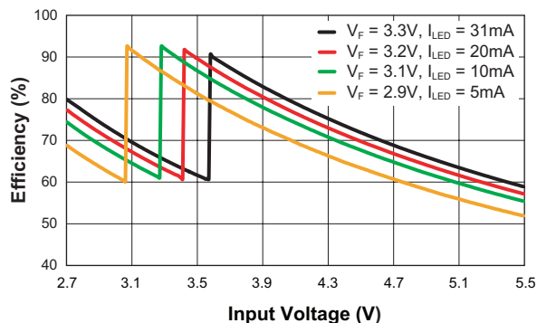
CP Efficiency vs. Input Voltage
